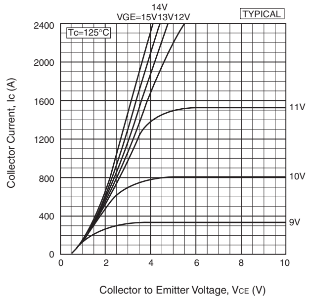
Collector current vs. Collector to Emitter voltage
