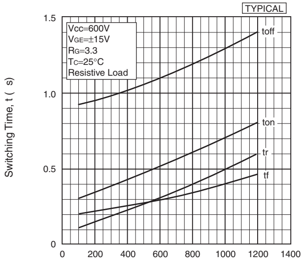
Switching time vs. Collector current
