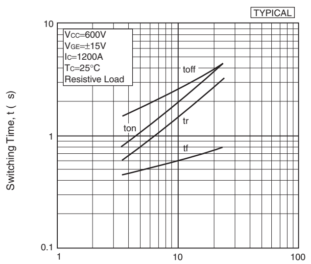
Switching time vs. Gate resistance
