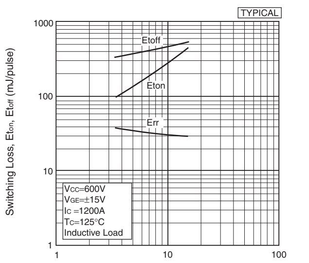
Switching loss vs. Gate resistance
